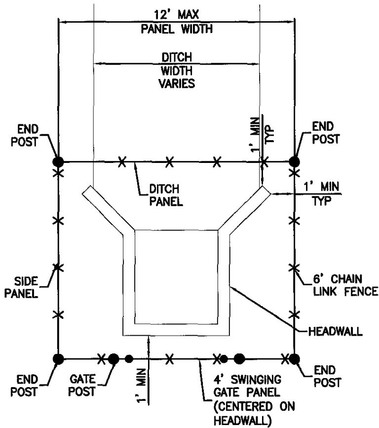
PLAN VIEW
