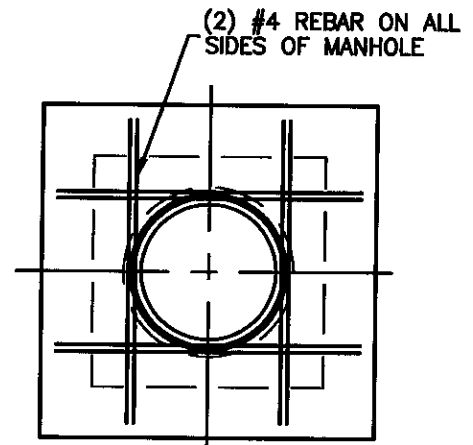
TOP SLAB REINFORCING PLAN
