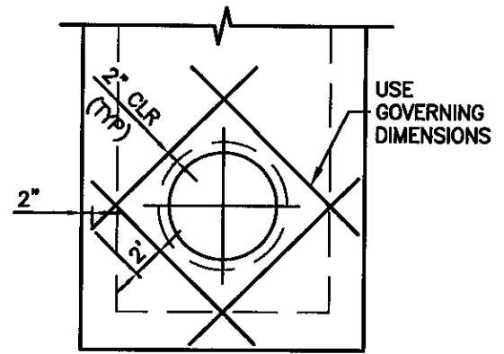
TOP SLAB REINFORCING PLAN
